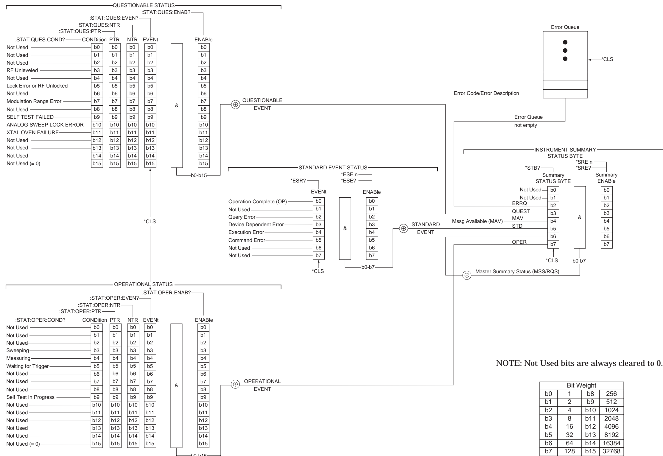
Figure 2-1. 683XXC Status-Reporting Structure
