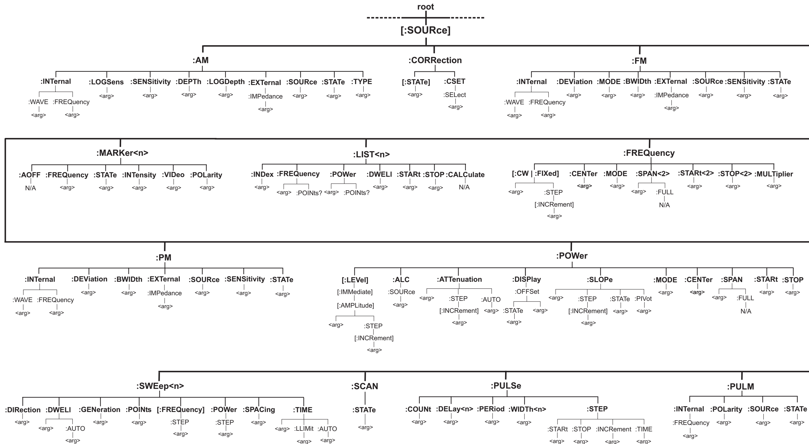
Figure A-1. Overall 683XXC SCPI Command Tree (Sheet 2 of 2)
